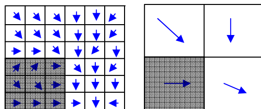
Figure 8. The effect of DEM resolution on flow vectors; left 5 m. and right 15 m. resolution
